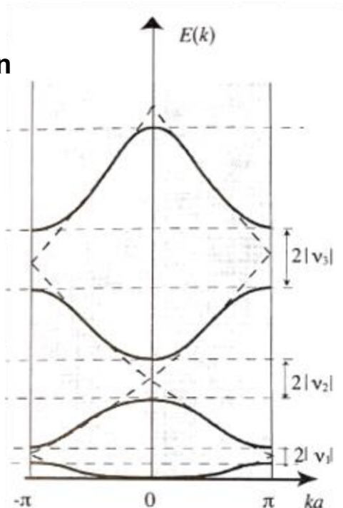
Periodic potential
